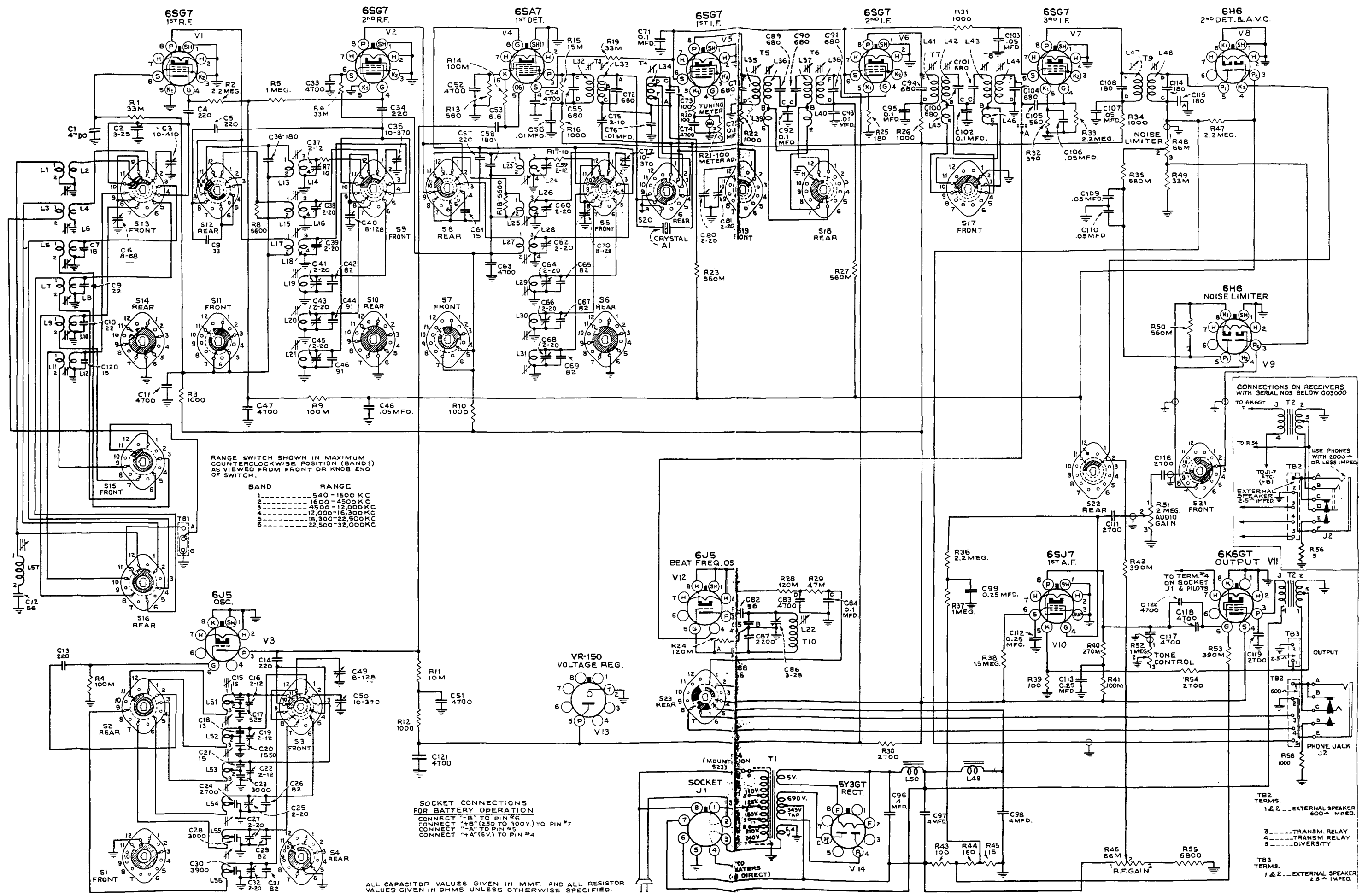
Figure 11—Schematic Diagram
