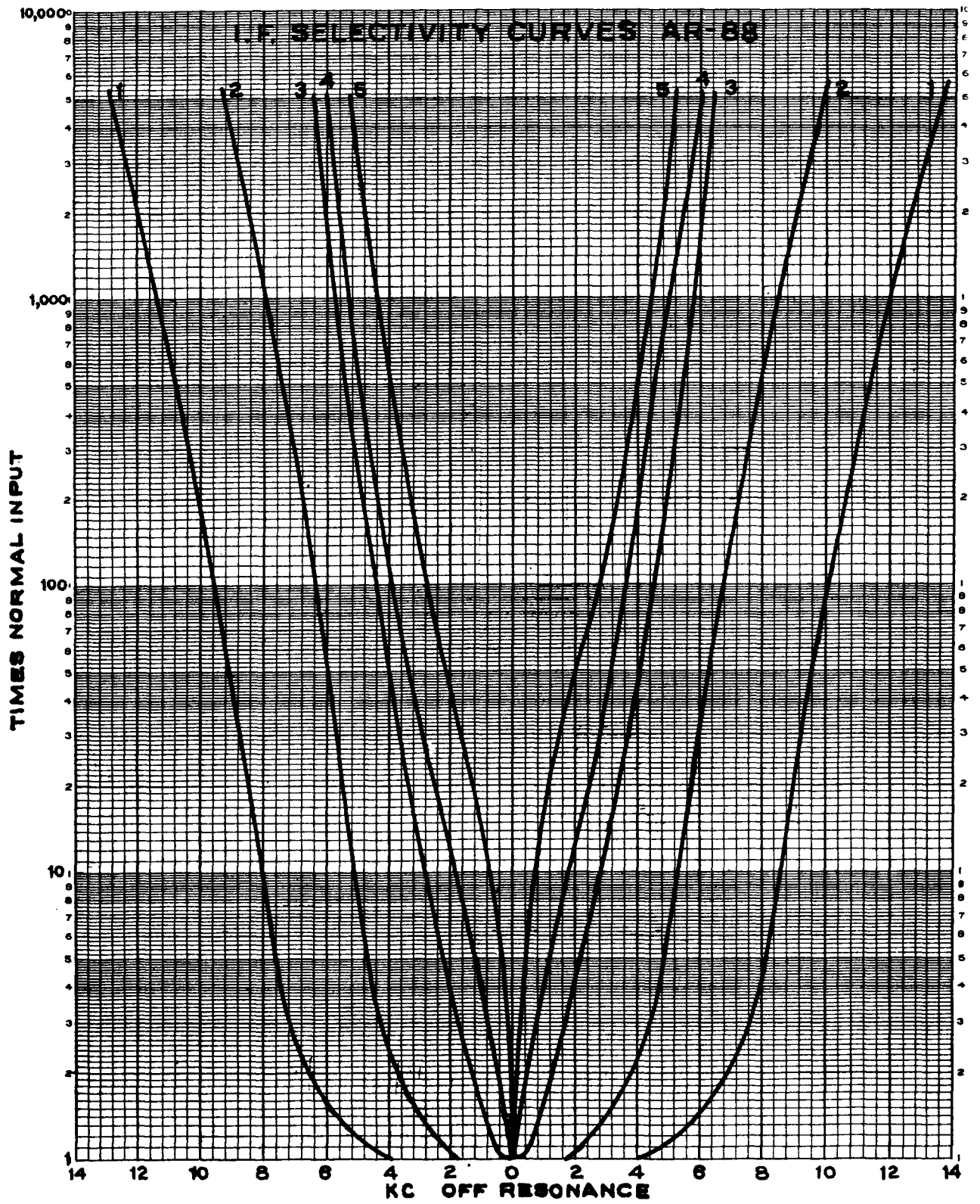
Figure 12—Selectivity Curves
