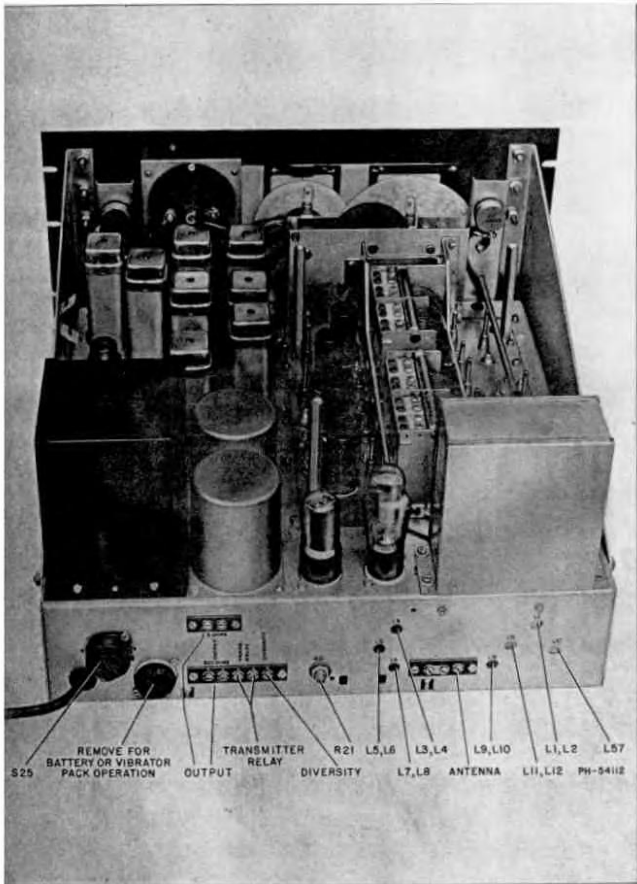
Figure 6—AR-88 Chassis
