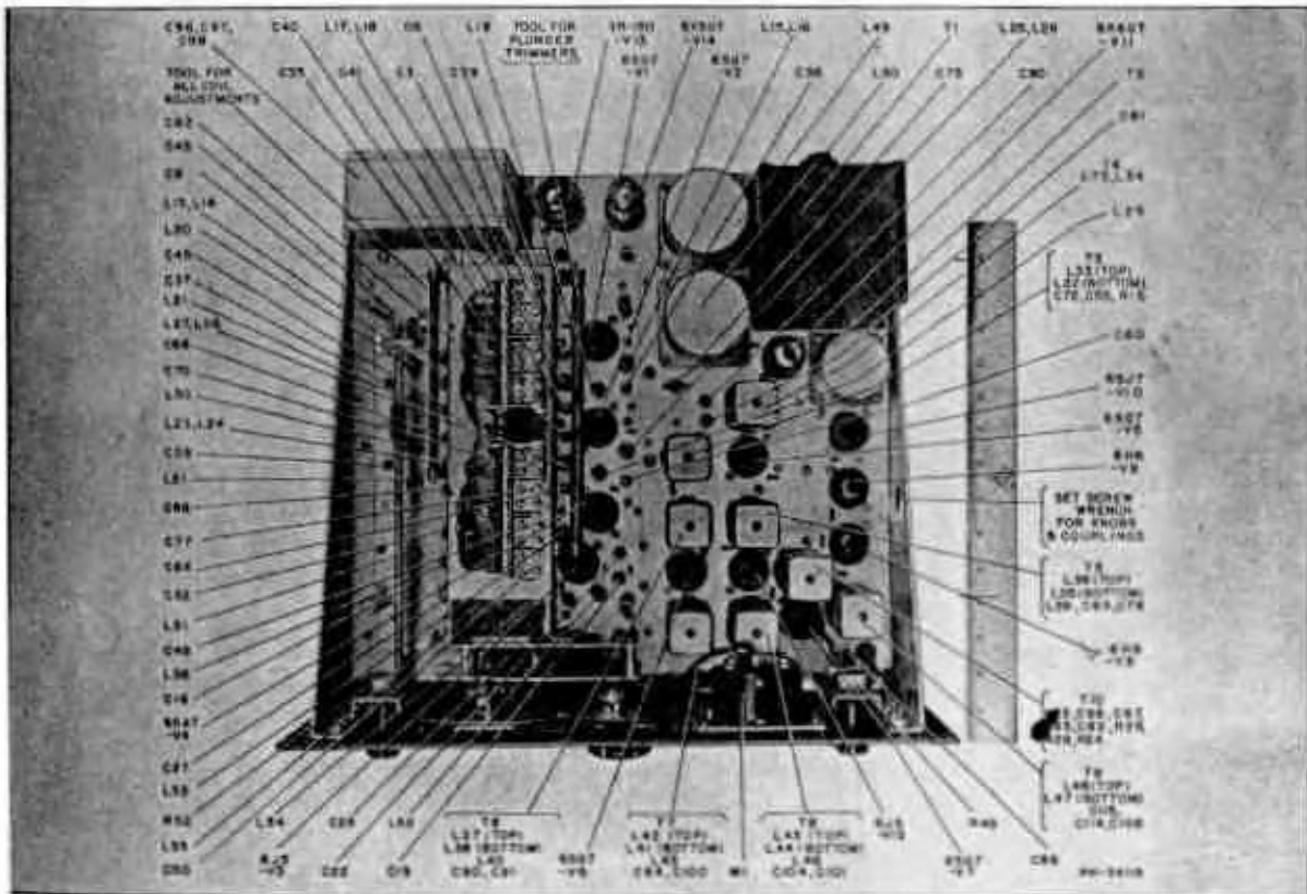
Figure 8—Top View of Chassis—Covers Removed
